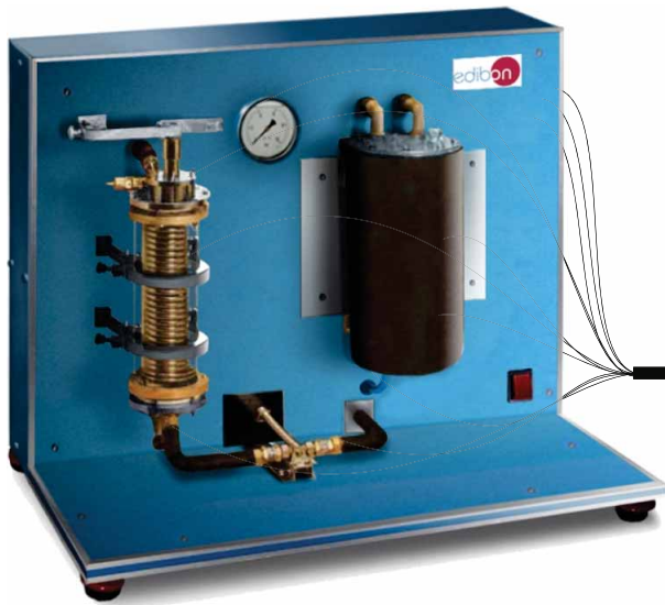
① Unit: HTVC. Solar/Heat Source Vapour Turbine
